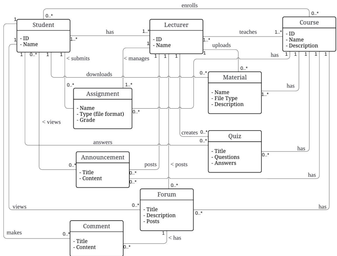
Figure 1 Domain Model of UKMFolio
